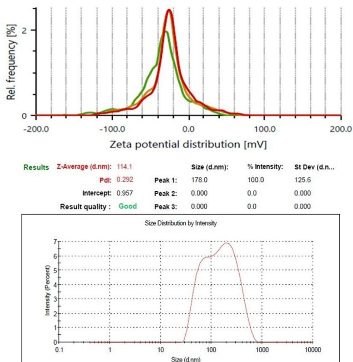
Figure 4.43: Zeta potential and particle size distribution results of optimized transferosomes (formulation BDT-10) stored at 25±2 °C/ 60±5 % RH for 3 months.
