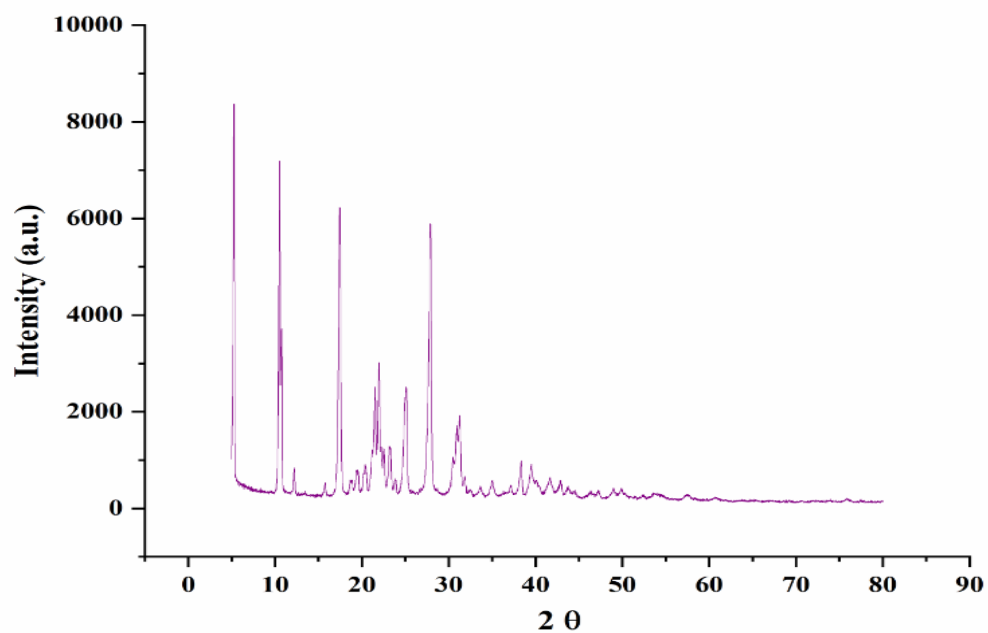
Figure 4.19: X-ray diffraction spectrum of diacerein.
