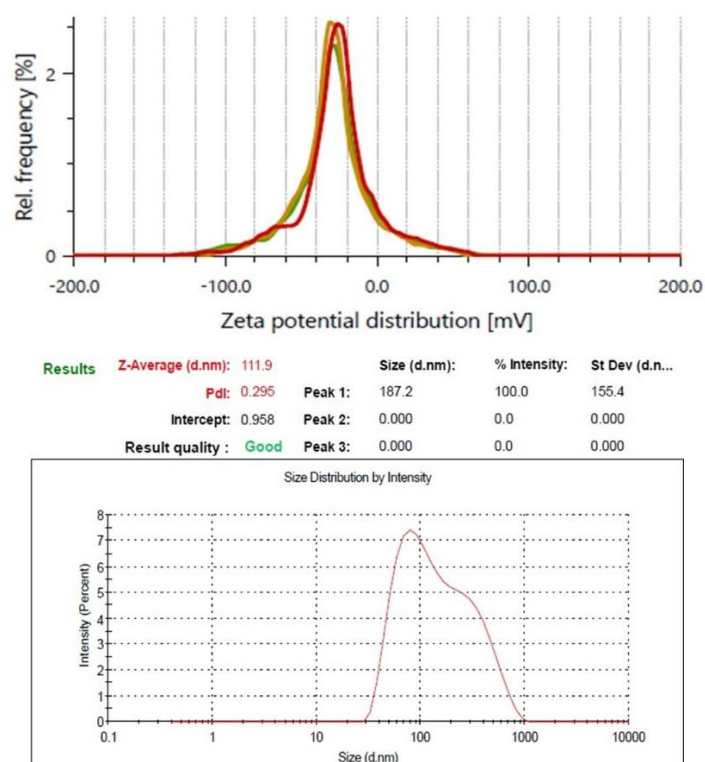
Figure 4.42: Zeta potential and particle size distribution results of optimized transferosomes (formulation BDT-10) stored for 3 months at 4±1 °C.
