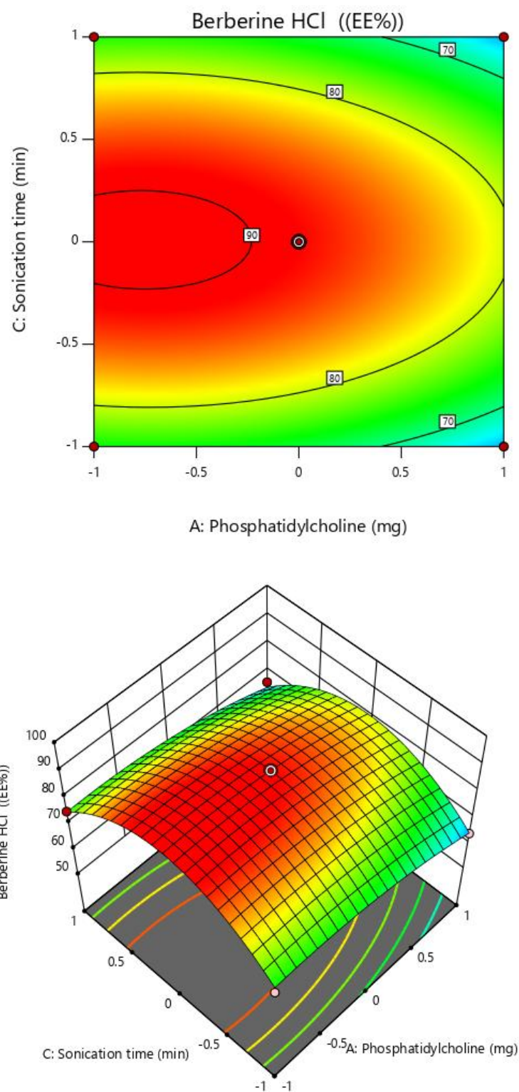
Figure 4.9. 3D response surface and contour plots illustrating the relationship between formulation variables (phosphatidylcholine concentration and sonication time) on percentage entrapment efficiency of berberine HCl.
