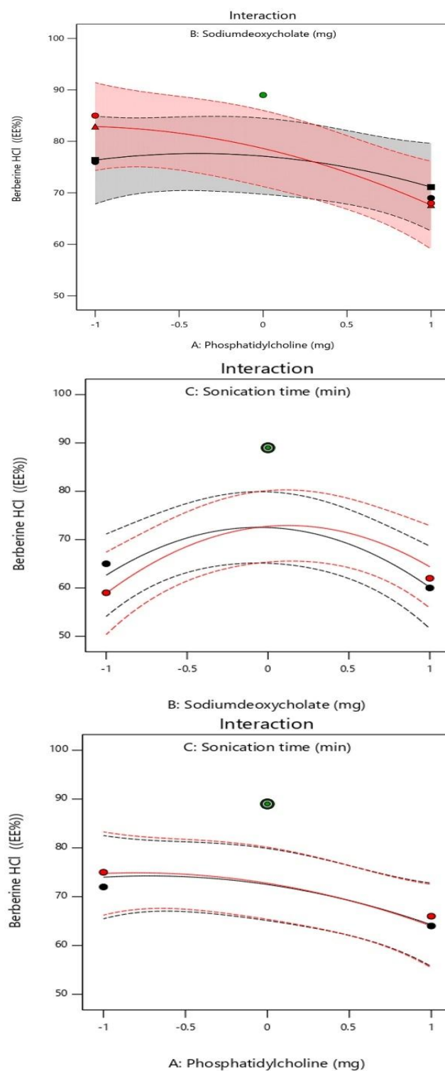
Figure 4.15. Interaction between the amount of edge activator (sodium deoxycholate) and phospholipid (phosphatidylcholine), amount of phospholipid and sonication time, and amount of edge activator and sonication time affecting entrapment of berberine HCl.
